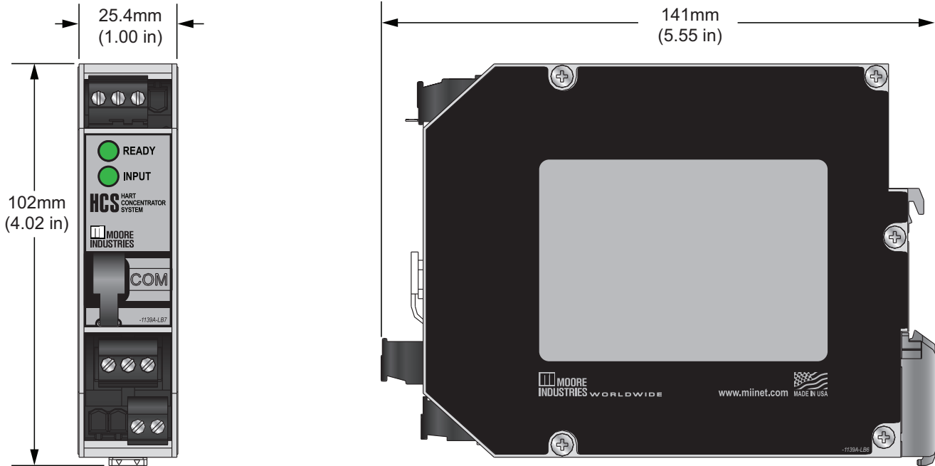
Figure 4. Installation Dimensions
