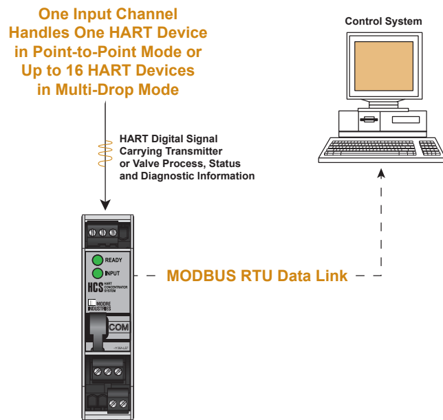
Figure 1. The HCS economically converts HART to serial MODBUS RTU (RS-485 or RS-232) protocol.
