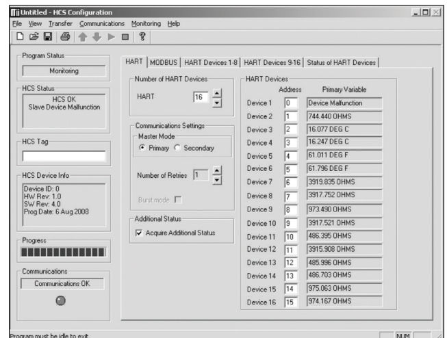
Figure 3. In just minutes, you can set up the HCS using our single window Intelligent PC Configuration Software.
